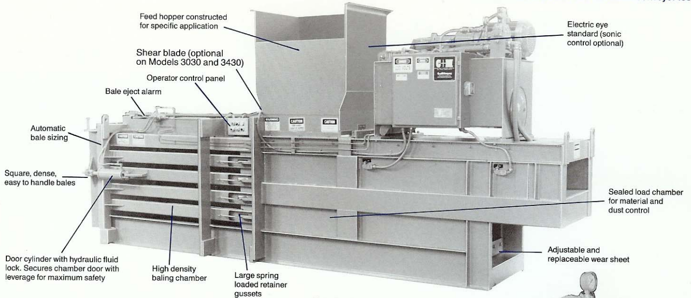
C+M Model 3430-7256 with conveyor feed hopper
