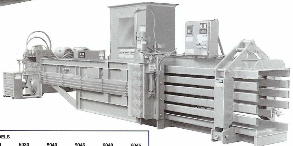
C+M Model 5030-AT510
